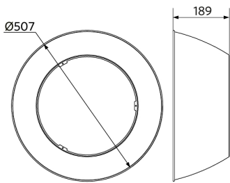
LEDHighbay-E2 Bracket
