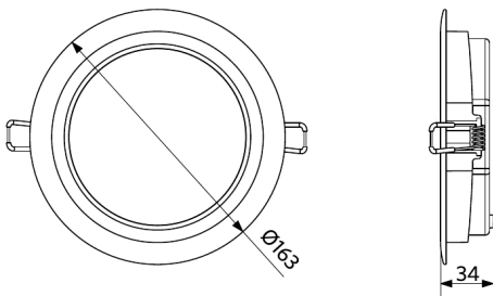
LEDDownlightRc-SI-E Rd150
