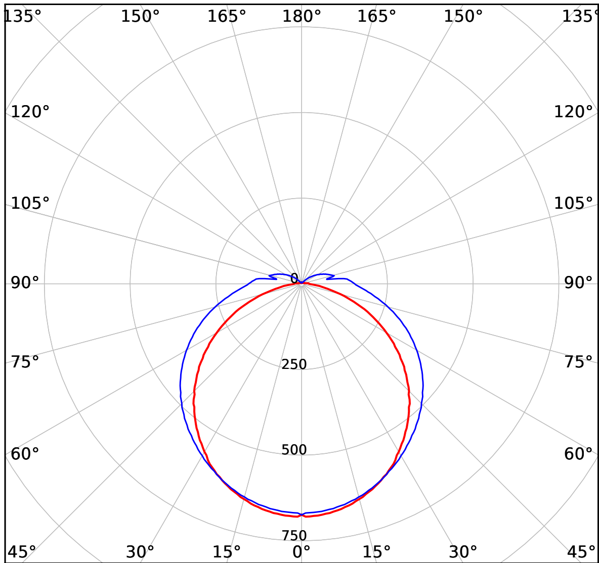
cd 2500 lm — C0-C180 — C90-C270
