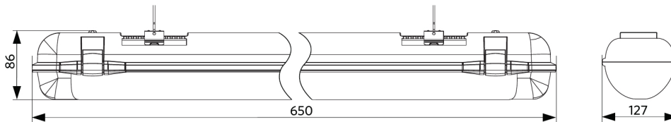
LEDWaterproof-CLA-E L1250
