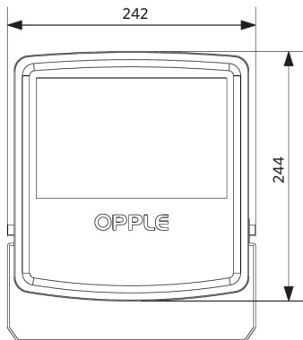
LEDflood-E-Re250-280-Bracket
