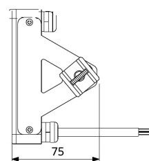
LEDflood-E Sensor
