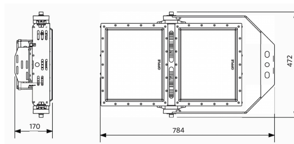
LEDfloodHO-P-620W (+MountingKit-2Mod)
