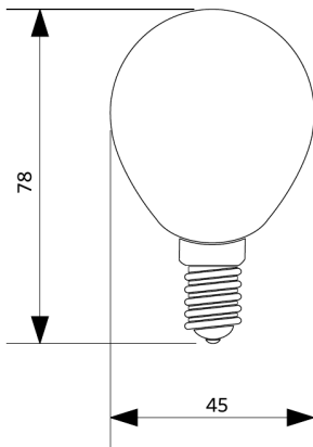
LED-E-P45-FILA
