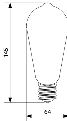
LED-E-ST64-FILA
